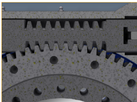
Direct drive with worm shaft
